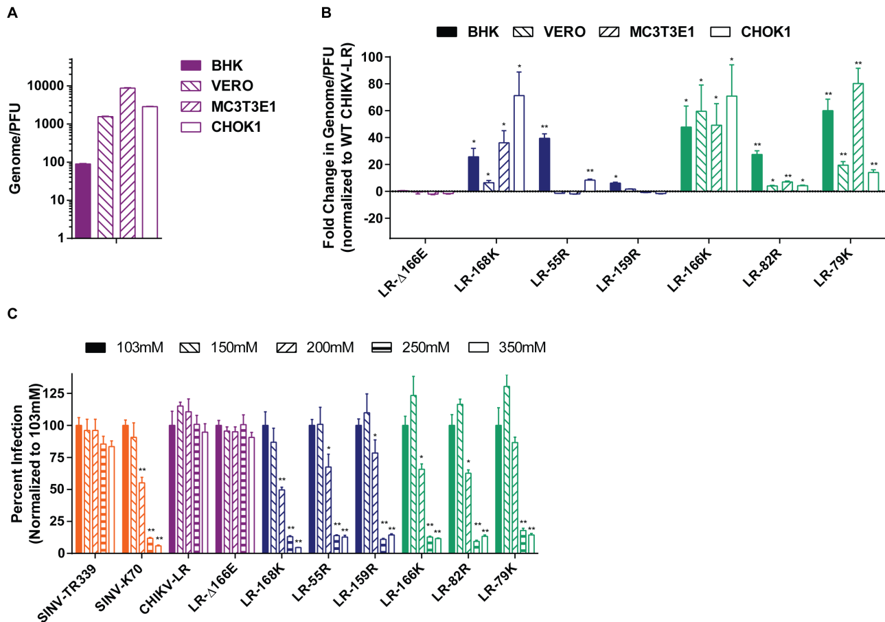
Figure 5. Positive charge CHIKV E2 mutations increase specific infectivity and infectivity is dependent on ionic interactions. Specific infectivity (GE/PUF) of A) CHIKV-LR WT; and B) the mutants CHIKV E2 mutants were evaluated on different cell types. For the CHIKV E2 mutants, fold-change in specific infectivity was normalized to CHIKV-LR. C) CHIKV E2 mutants were evaluated for dependency on ionic interaction for infectivity by interacting virus in either RPMI1640 (basal salt concentration of 103 mM NaCl) or RPMI1640 with increasing salt concentration and MC3T3-E1 cells were then infected for a standard plaque assay. Percent infectivity was normalized to 103 mM NaCl, which was set to 100%. Viruses are color-coded based on control groups (orange) or MSD severity: little or no attenuation (purple), partial attenuation (blue) or highly attenuated (green) compared to CHIKV-LR. Error bars represent standard deviation. * p < 0.01 and ** p < 0.001 compared to CHIKV-LR (B) or 103 mM NaCl (C). doi:10.1371/journal.pntd.0002719.g005
